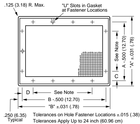
Figure C Shielded Air Filters, Standard Construction
