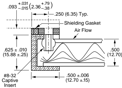
Figure A Standard Frame Design 61-118
