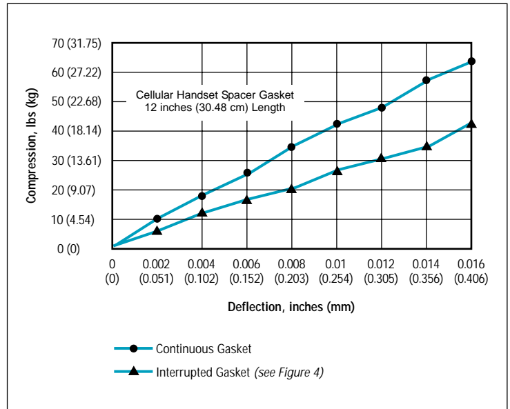
Figure 5 Typical Spacer Gasket Deflection
