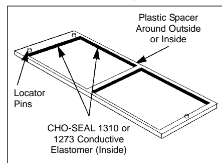
Figure 1 Single Piece EMI Gasket/Plastic Spacer for Accurate and Low Cost Installation
