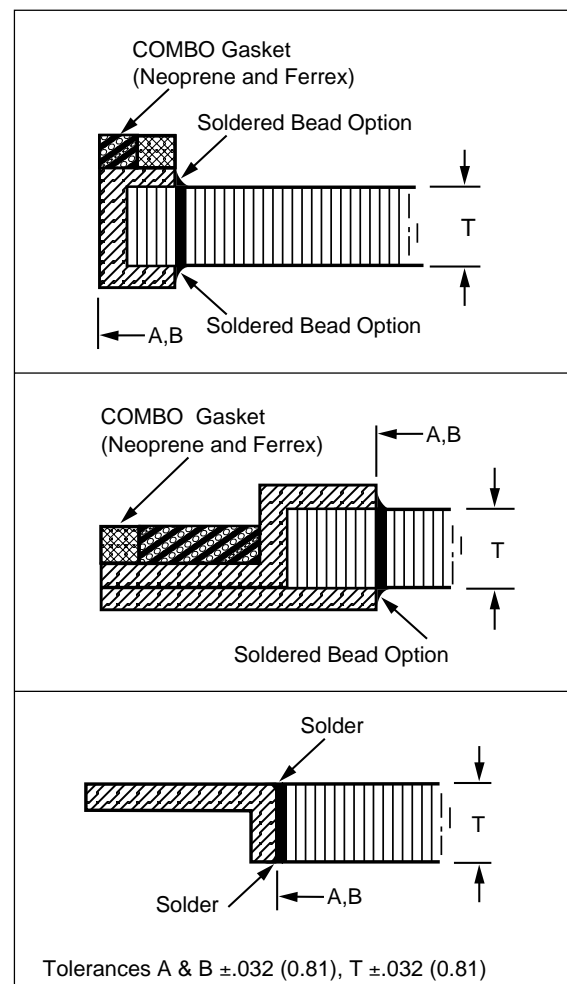
Figure A Typical Frame Styles (others available)
