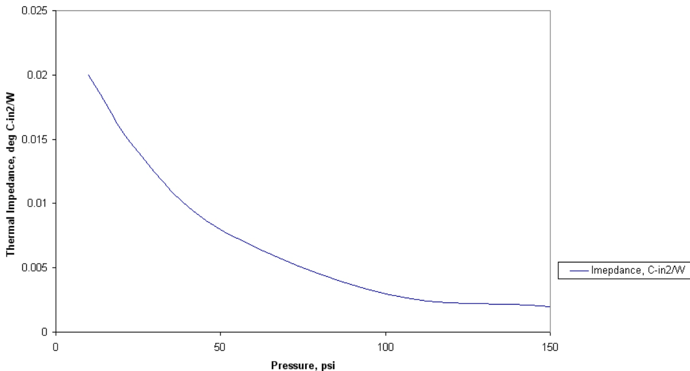
T557 Impedance vs Pressure tested at 70 deg C per ASTM D5470
