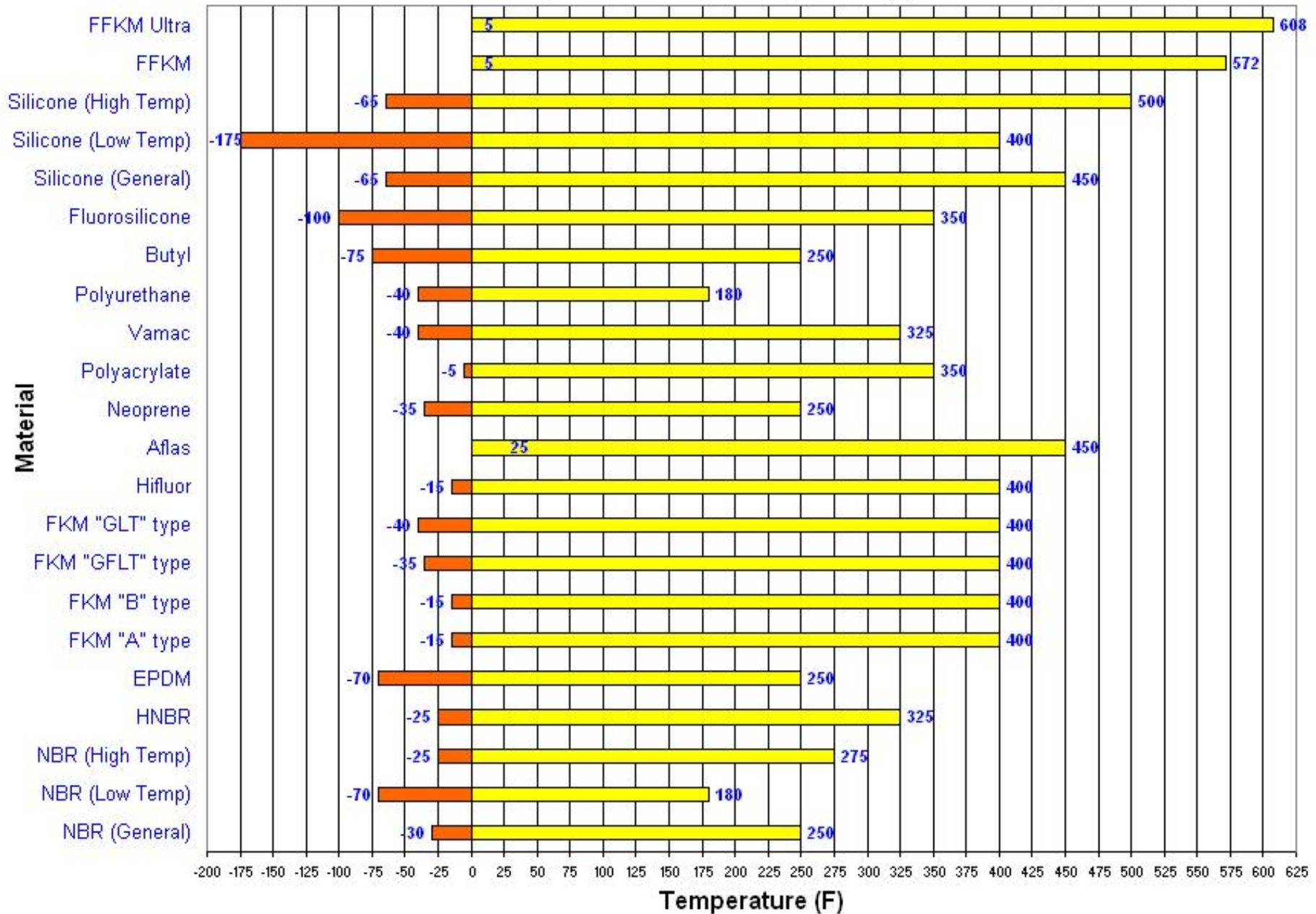
Material Temperature Range Comparison (F)
