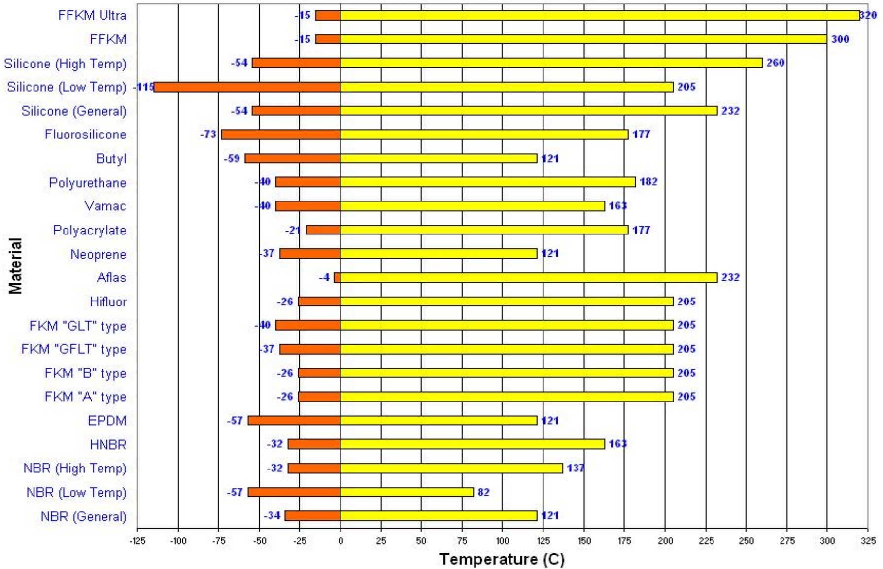
Material Temperature Range Comparison (C)
